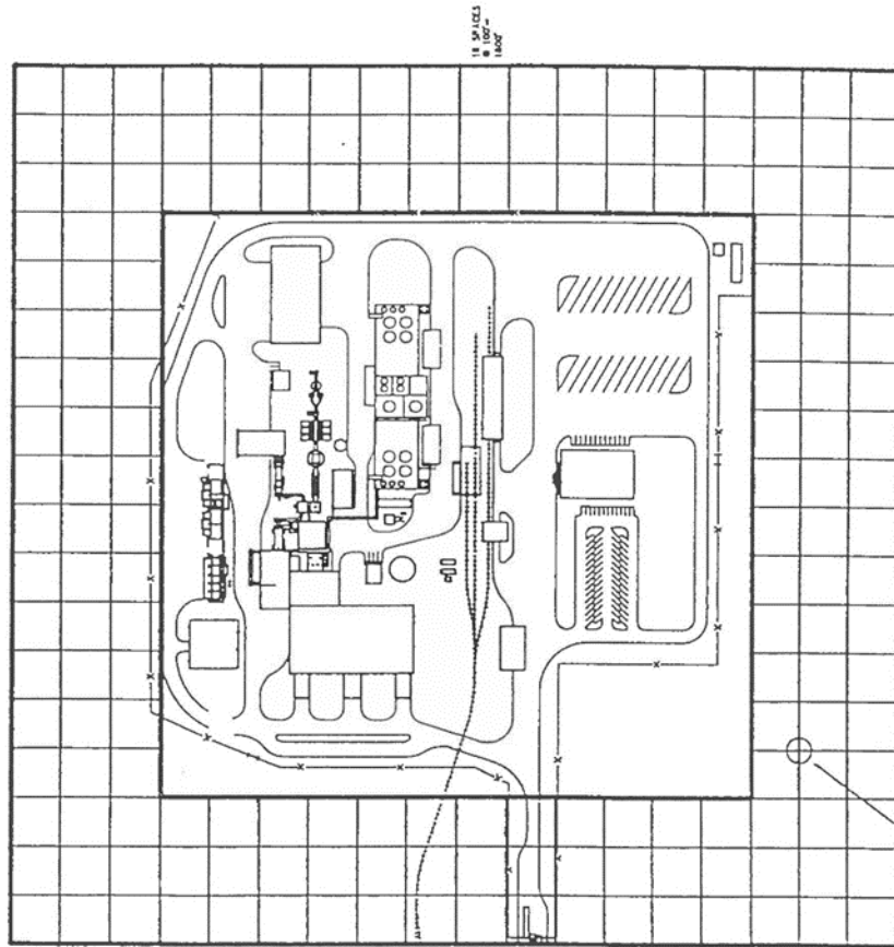
16 SQUARES = 100'-100' FIGURE 1-C-3 SOILS SAMPLING GRID EXTERNAL TO THE FACILITY PROPER (TYP) (REFER TO APPENDIX L.C. SECTION J.4) CLIVE INCINERATION FACILITY
